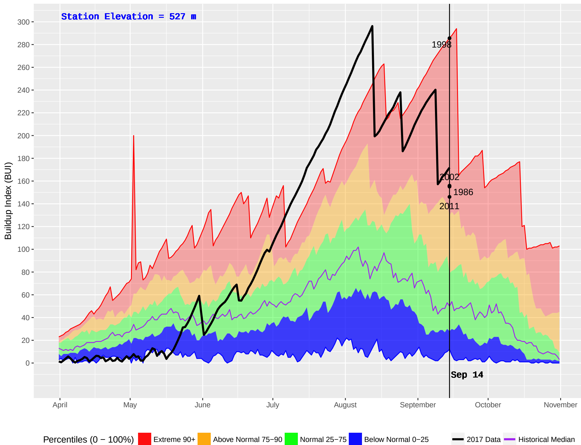
SALMON ARM (346) : Historical (1976–2016) and Current (2017) Noon Buildup Index (BUI)
