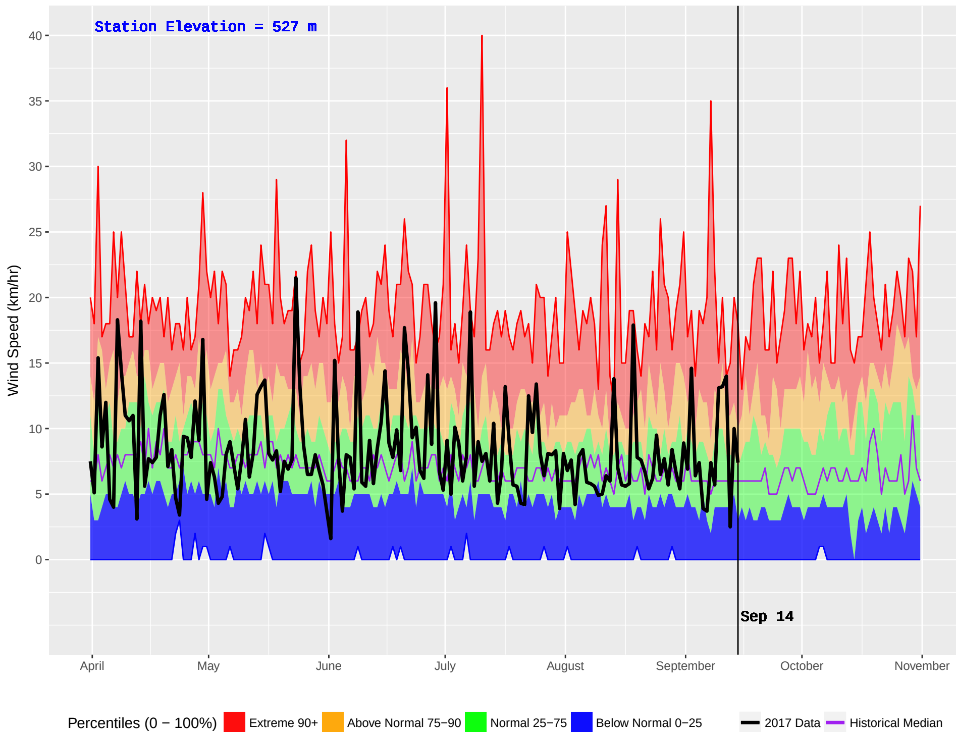
SALMON ARM (346) : Historical (1976–2016) and Current (2017) Noon Wind Speed
