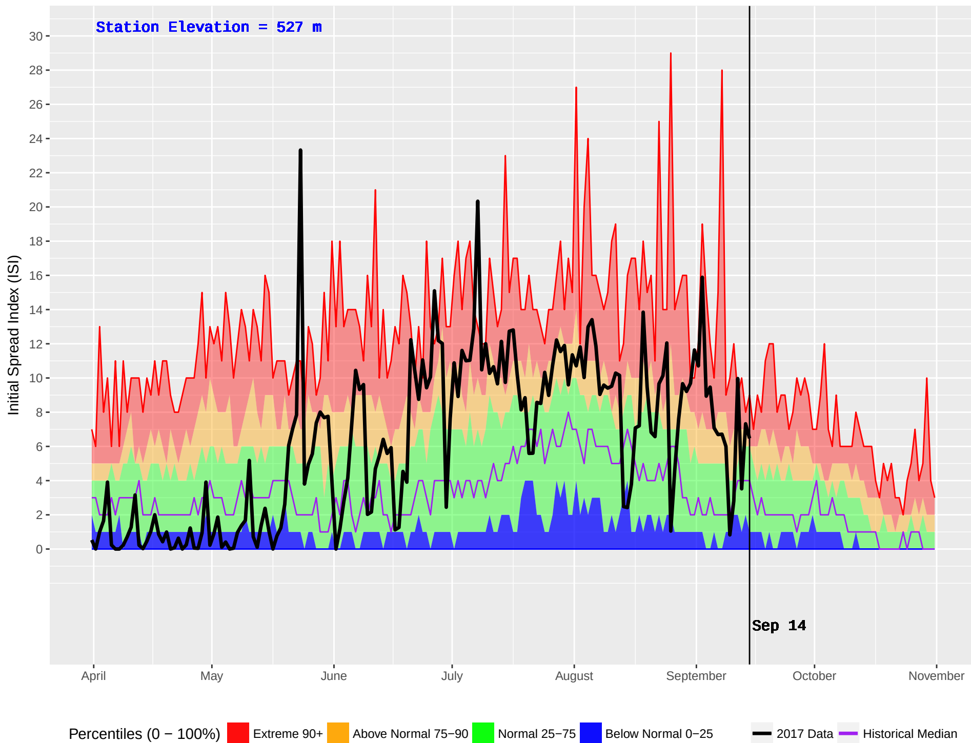
SALMON ARM (346) : Historical (1976–2016) and Current (2017) Noon Initial Spread Index (ISI)
