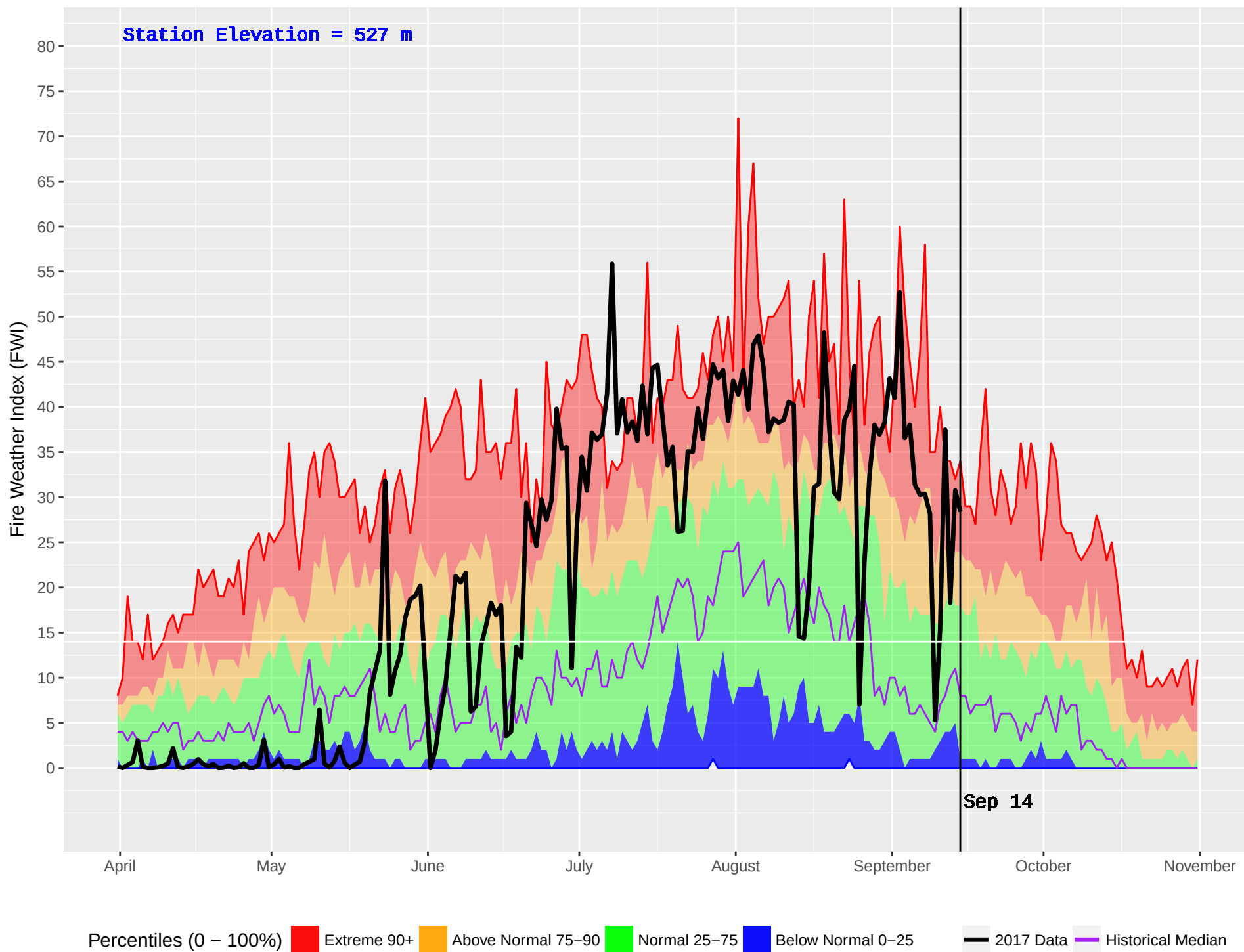
SALMON ARM (346) : Historical (1976–2016) and Current (2017) Noon Fire Weather Index (FWI)
