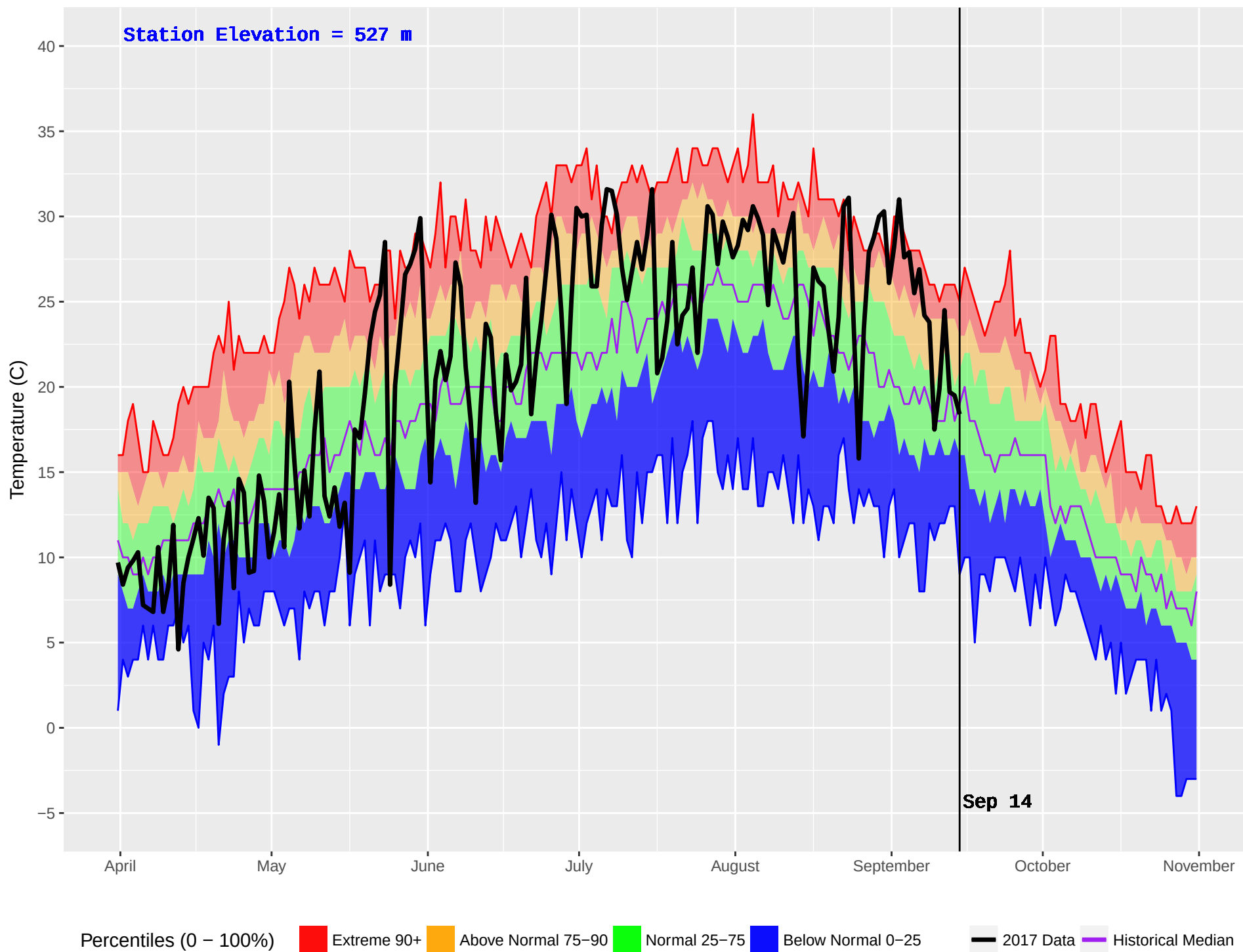
SALMON ARM (346) : Historical (1976–2016) and Current (2017) Noon Temperature
