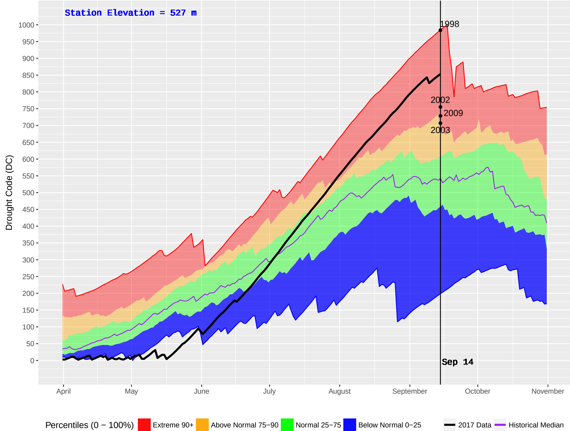
SALMON ARM (346) : Historical (1976–2016) and Current (2017) Noon Drought Code (DC)
